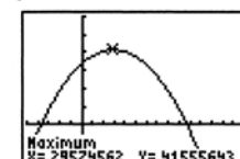
[-0.5, 1.5] by [-0.2, 0.6]
