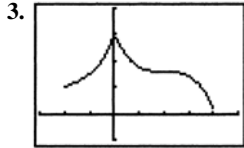
[-3, 5] by [-5, 20]
