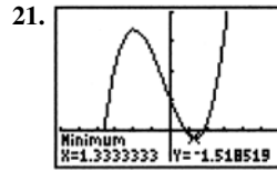
[-6, 6] by [-5, 20]
