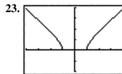
[-4, 4] by [-2, 4]
