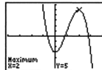
[-4, 4] by [-6, 6]
