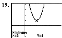
[-2, 6] by [-2, 4]
