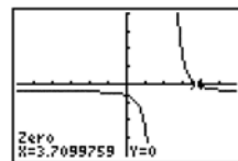
[-5.875, 5.875] by [-20, 20]
