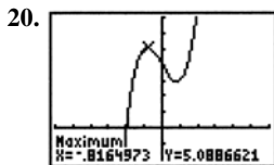
[-6, 6] by [-2, 7]
